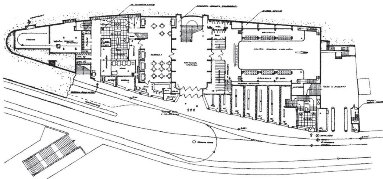
Josip Pičman, Narodni dom u Sušaku, tlocrt niskog prizemlja s glavnim ulazima, centralnim vestibulom i galerijom kupališta, 1935. g. Josip Pičman, Cultural Centre in Sušak, ground plan of the lower ground floor with the main entrance doors, central vestibule, and the gallery of the swimming pool, 1935
