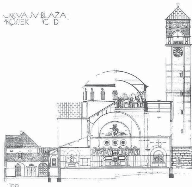
8 Viktor Kovačić, poprečni presjek C-D kroz crkvu, listopad 1909. g. / 24.08.1910. g. / Viktor Kovačić, C-D cross section of the church, October 1909/24th August 1910
